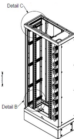
ISOMETRIC VIEW M 1:15
