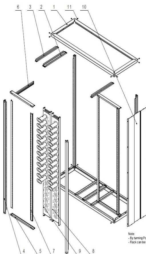
EXPLODED VIEW M 1:12.5
